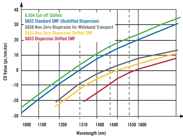
Figure 2: Expected CD values based on fiber type
