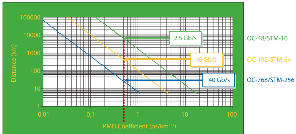
Figure 1: Maximum distance vs. PMD coefficient and bit rate
