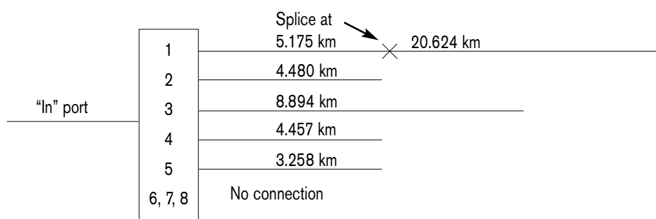
Figure 4: Logical layout of example #1
