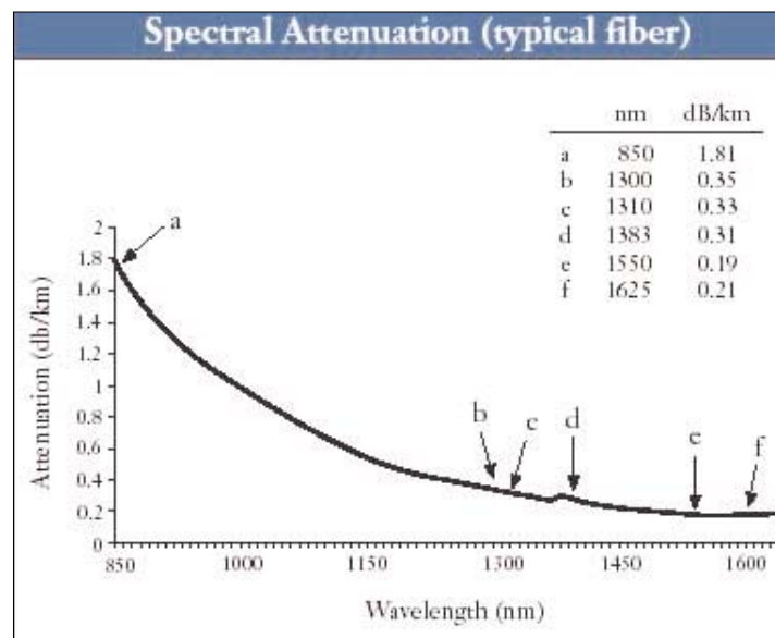
Figure 2: Attenuation per \lambda on typical G.652C fiber Source: Corning's SMF-28e spec sheet, July 2003
