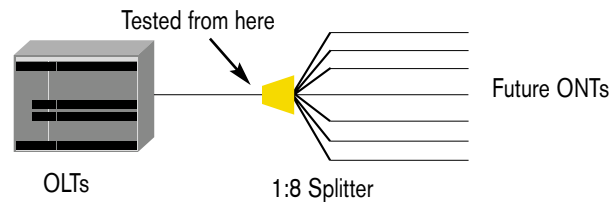
Figure 3: Installation example: 1 x 8 splitter, 5 fibers terminated
