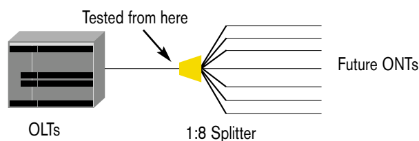
Figure 3: Installation example: 1 x 8 splitter, 5 fibers terminated
